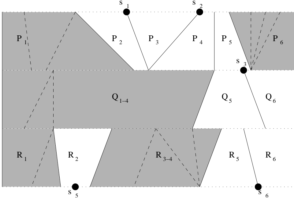
Fig. 3. Removal of s_4 from Figure 2.
