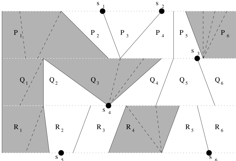
Fig. 2. A visibility representation and an underlying drawing.
