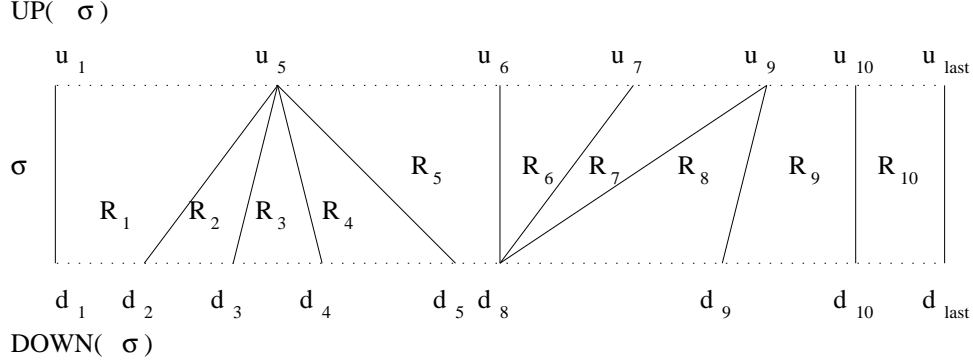
Fig. 1. Upward and downward projections of a sequence of visibility regions.
